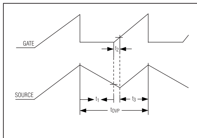
Figure 8. MAX15008 Timing Diagram
