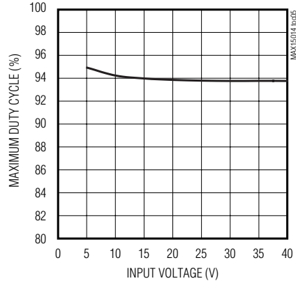
MAXIMUM DUTY CYCLE vs. INPUT VOLTAGE (MAX15015A)
