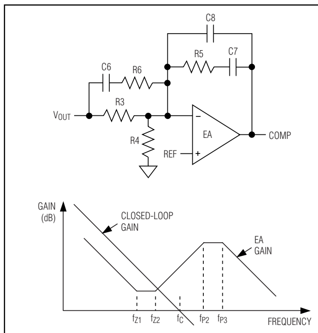
Figure 3. Error Amplifier Compensation Circuit (Closed-Loop and Error-Amplifier Gain Plot) for Ceramic Capacitors
