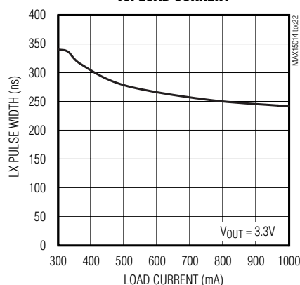
MINIMUM LX PULSE WIDTH vs. LOAD CURRENT
