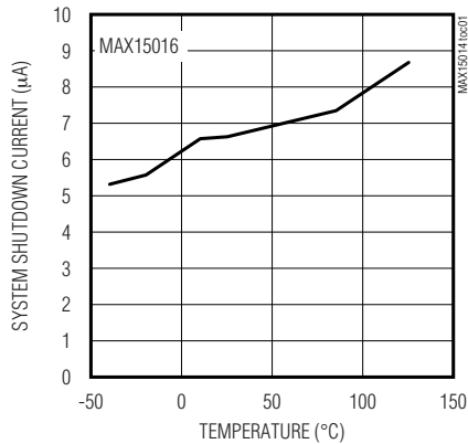
SYSTEM SHUTDOWN CURRENT vs. TEMPERATURE
