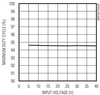
MAXIMUM DUTY CYCLE vs. INPUT VOLTAGE (MAX15016A)
