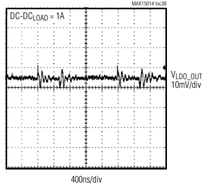
RESIDUAL SWITCHING NOISE ON THE LDO OUTPUT
