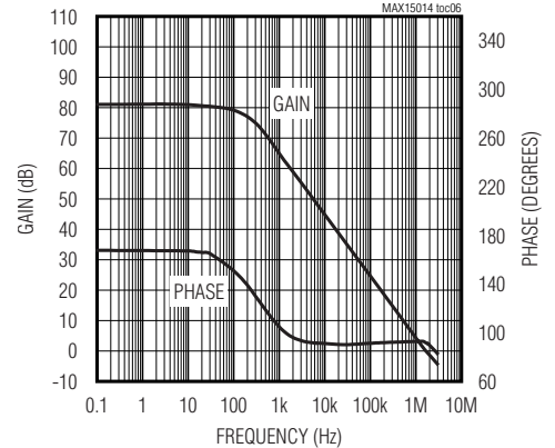
ERROR AMPLIFIER OPEN-LOOP GAIN AND PHASE vs. FREQUENCY
