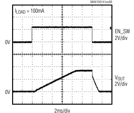
TURN-ON/OFF WAVEFORM
