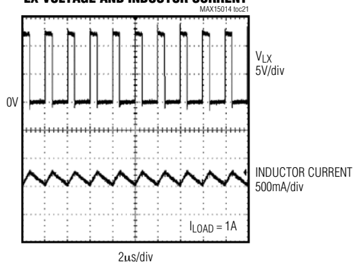
LX VOLTAGE AND INDUCTOR CURRENT
