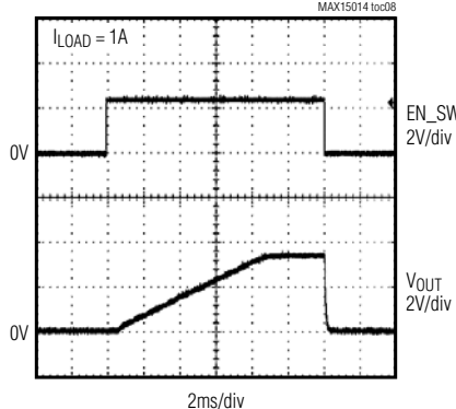
TURN-ON/OFF WAVEFORM
