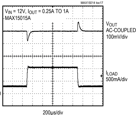
LOAD-TRANSIENT RESPONSE
