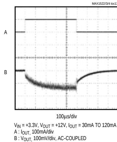
LOAD-TRANSIENT RESPONSE
