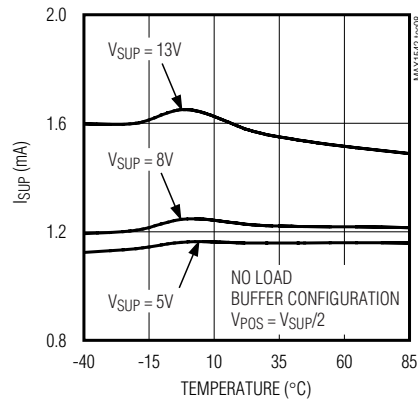
SUP SUPPLY CURRENT vs. TEMPERATURE
