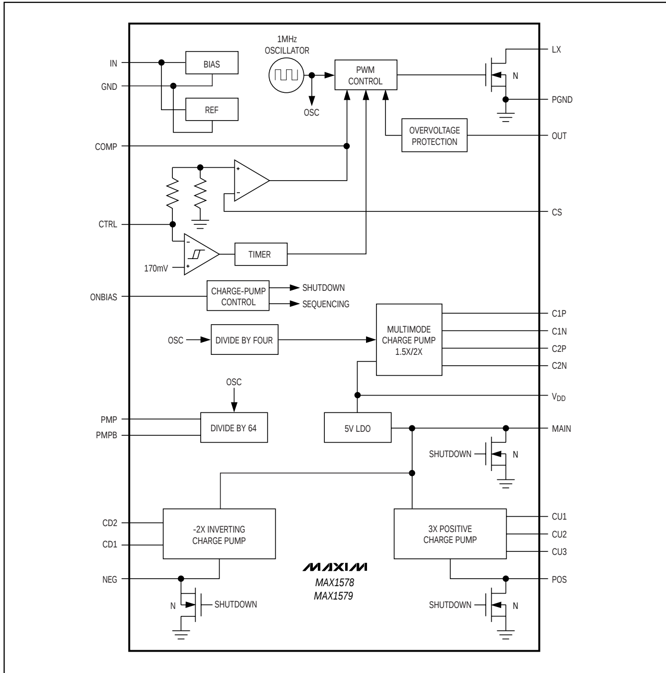
Block Diagram
