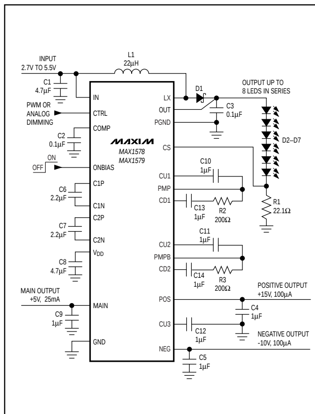
Figure 3. Typical Application Circuit
