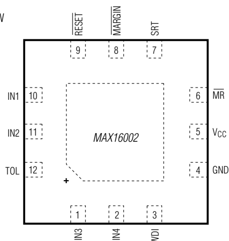
TQFN (4mm x 4mm)
