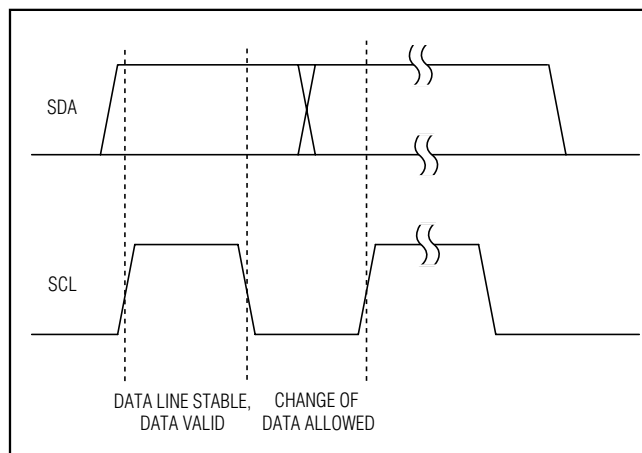
Figure 9. Bit Transfer
