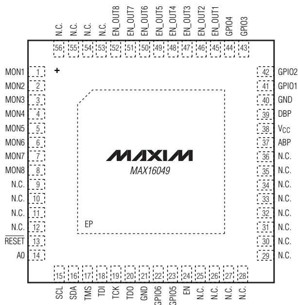
TQFN (8mm x 8mm)
