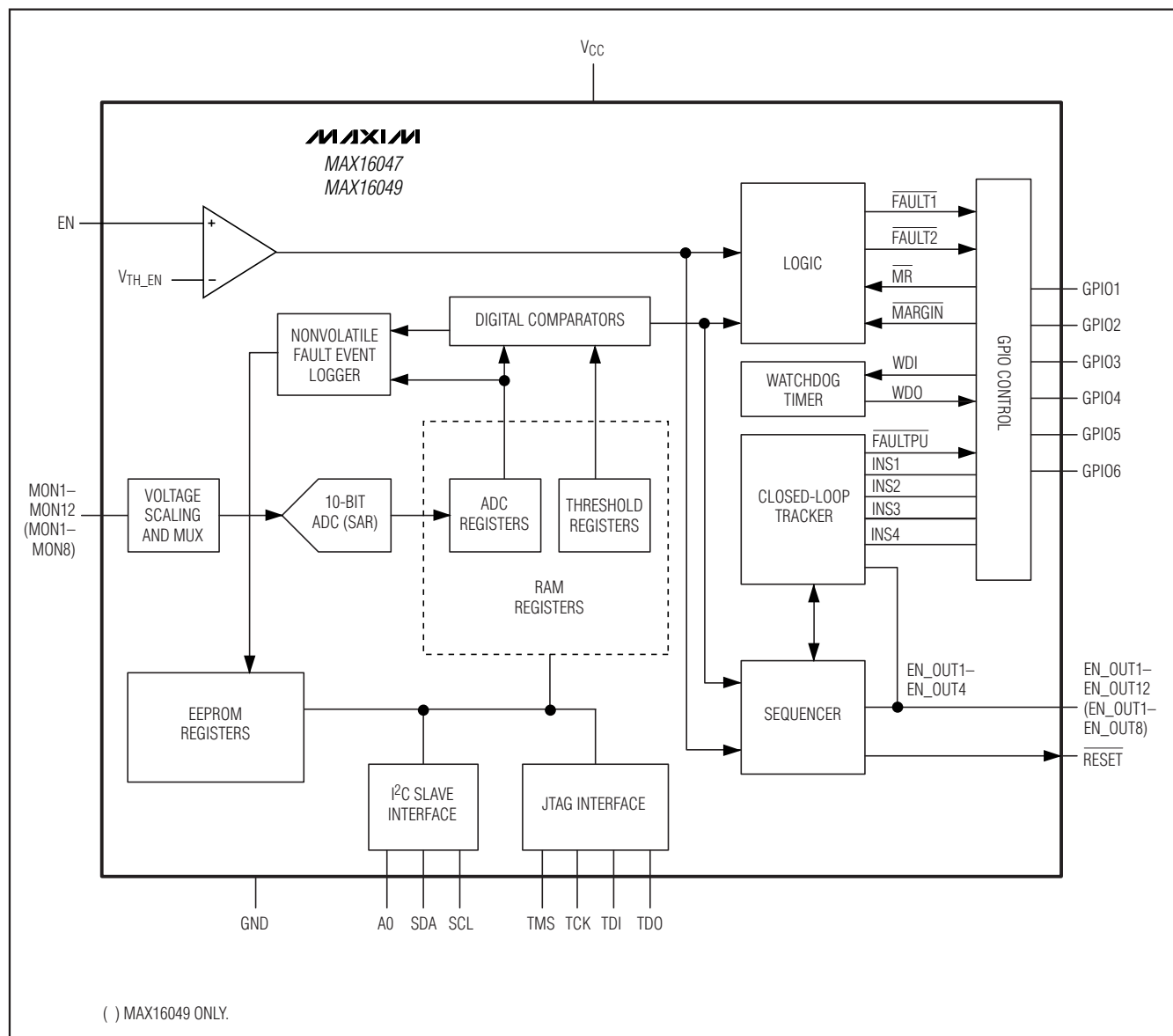
Functional Diagram
