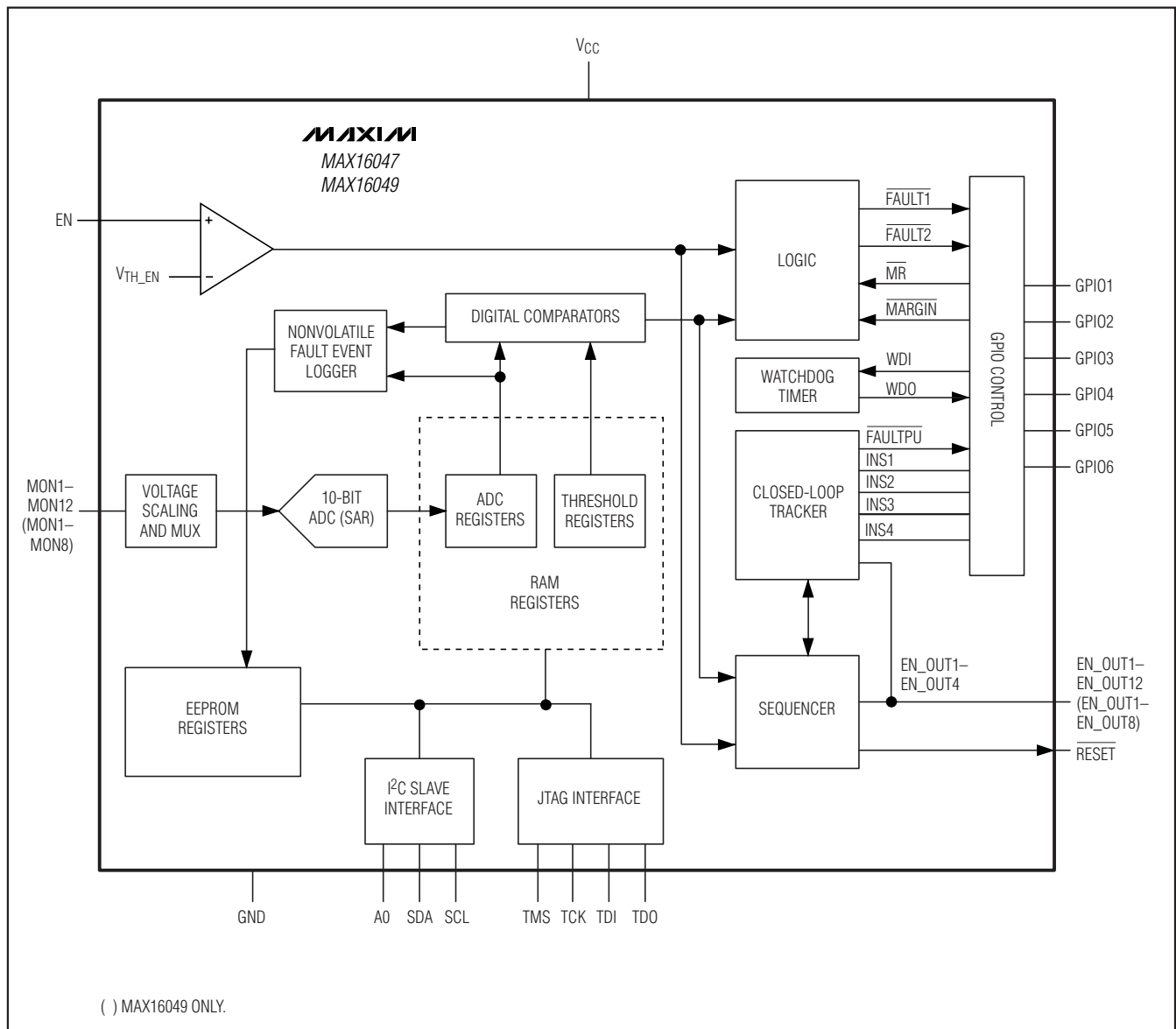
Functional Diagram
