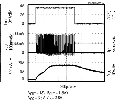
SHUTDOWN WAVEFORM
