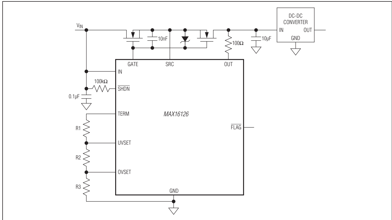
Figure 1. Overtolerance and Undervoltage Window Detector Circuit (MAX16126)
