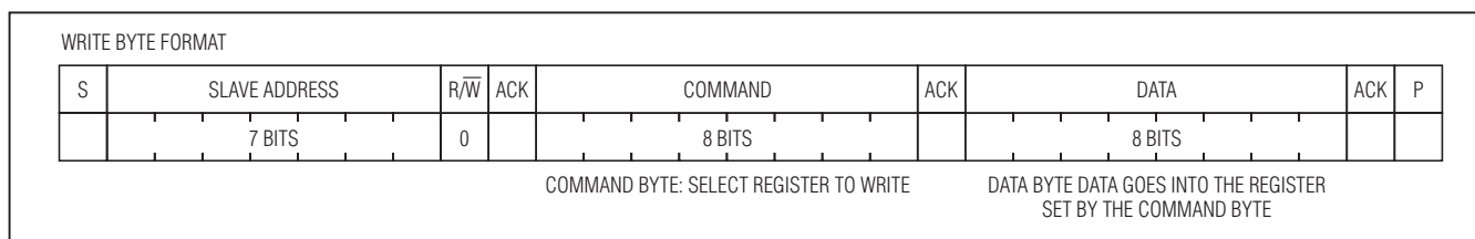
Figure 7. Write Byte Format
