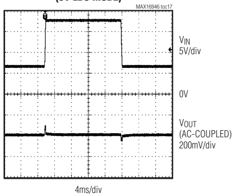
LINE TRANSIENT RESPONSE (5V LDO MODE)
