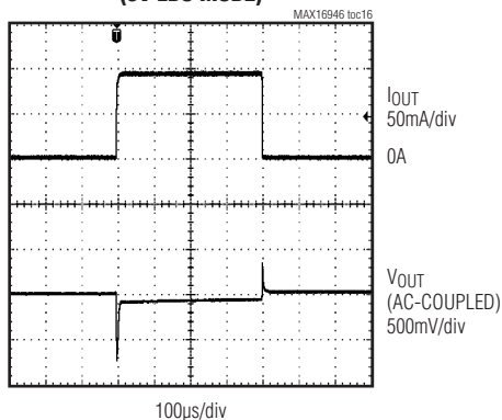
LOAD TRANSIENT RESPONSE (5V LDO MODE)
