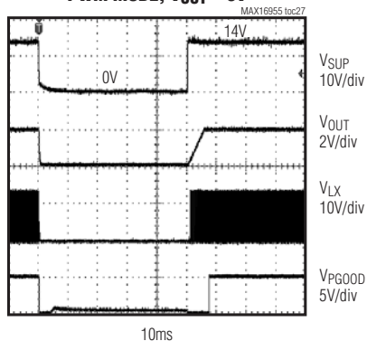
DIPS AND DROPS TEST, PWM MODE, V_{OUT} = 5V
