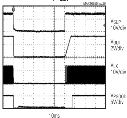
DIPS AND DROPS TEST, PWM MODE, V_{OUT} = 3.3V
