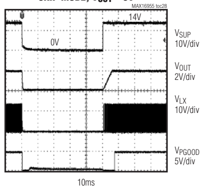
DIPS AND DROPS TEST, SKIP MODE, V_{OUT} = 5V
