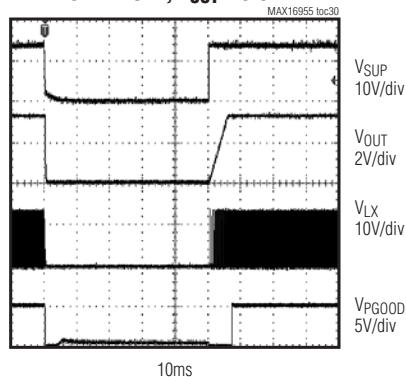
DIPS AND DROPS TEST, SKIP MODE, V_{OUT} = 3.3V
