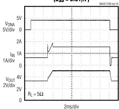
STARTUP WITH SOFT-START ( C_{SS} = 0.01\mu\text{F} )
