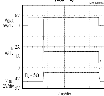
STARTUP WITHOUT SOFT-START ( C_{SS} = 0 )
