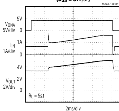
STARTUP WITH SOFT-START ( C_{SS} = 0.1\mu\text{F} )
