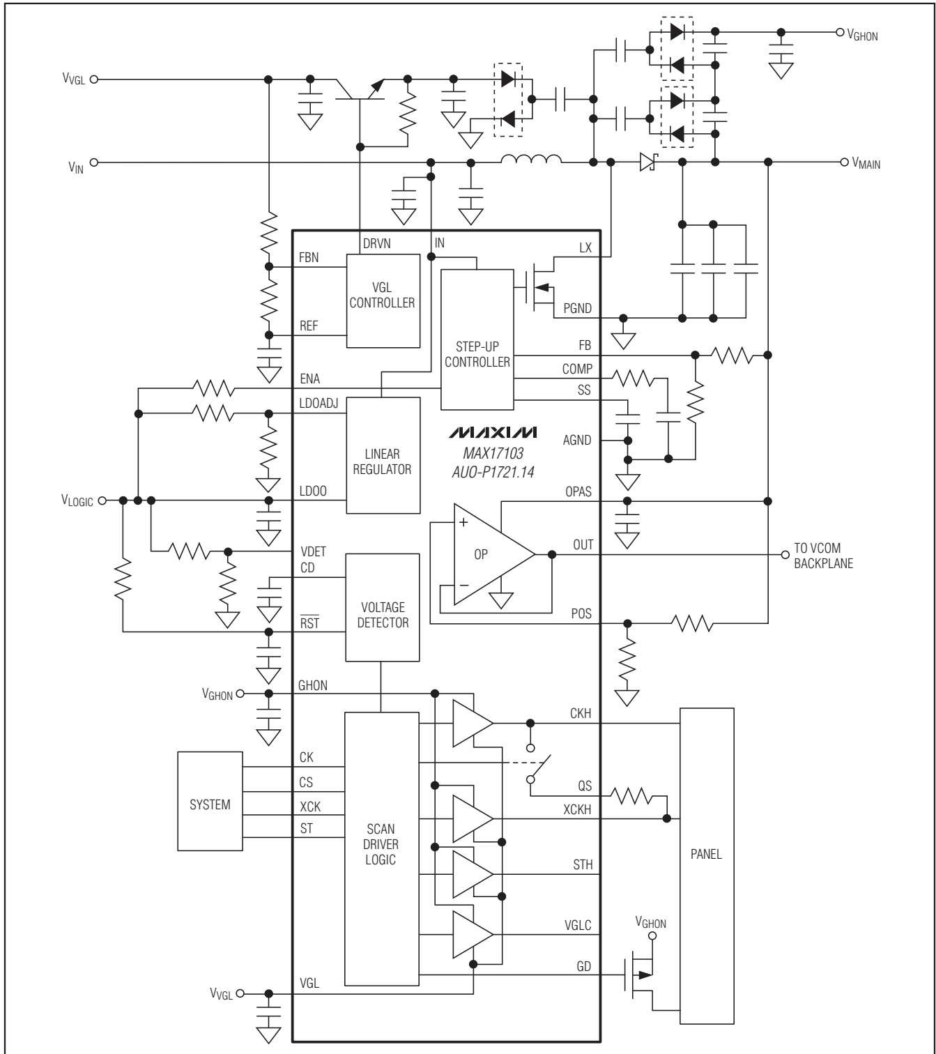
Figure 2. MAX17103 Functional Diagram
