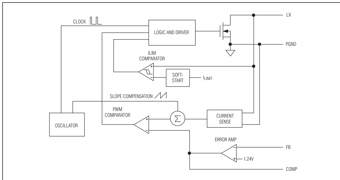
Figure 3. Step-Up Regulator Block Diagram
