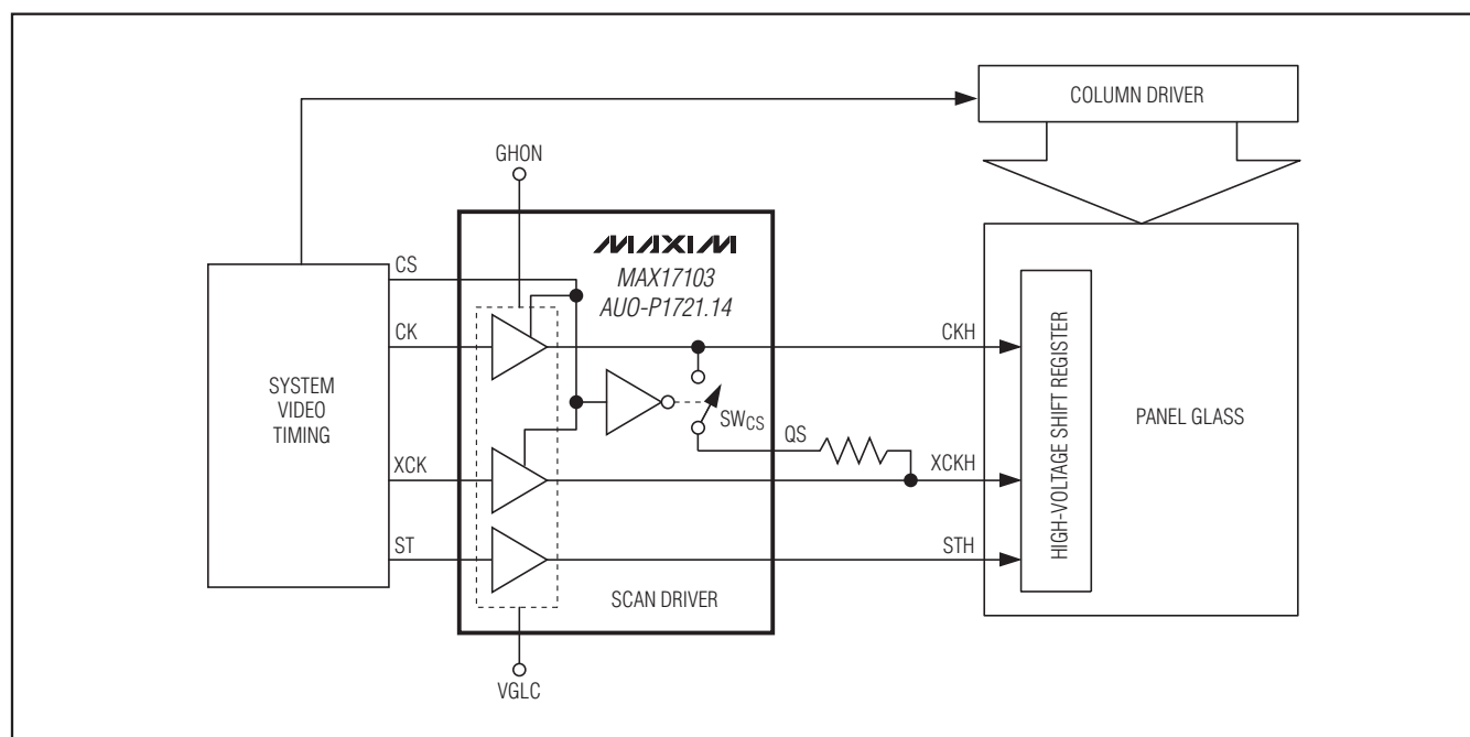
Figure 4. Scan Driver System Diagram
