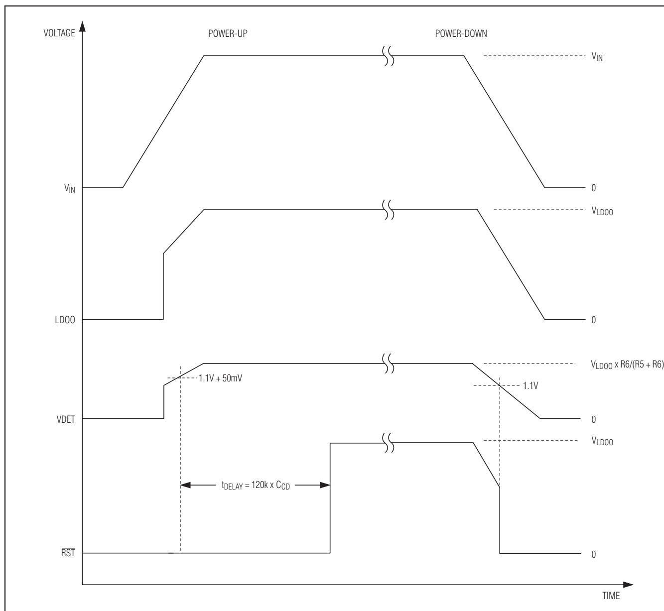
Figure 7. Voltage-Detector Power-Up and Power-Down Timing
