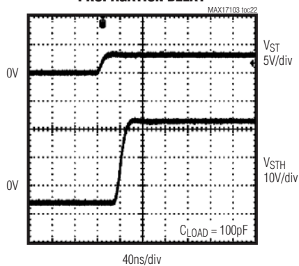
STH RISING EDGE PROPAGATION DELAY
