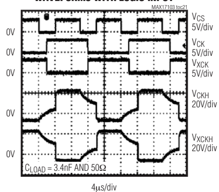
CKH AND XCKH OUTPUT WAVEFORMS WITH LOGIC INPUT
