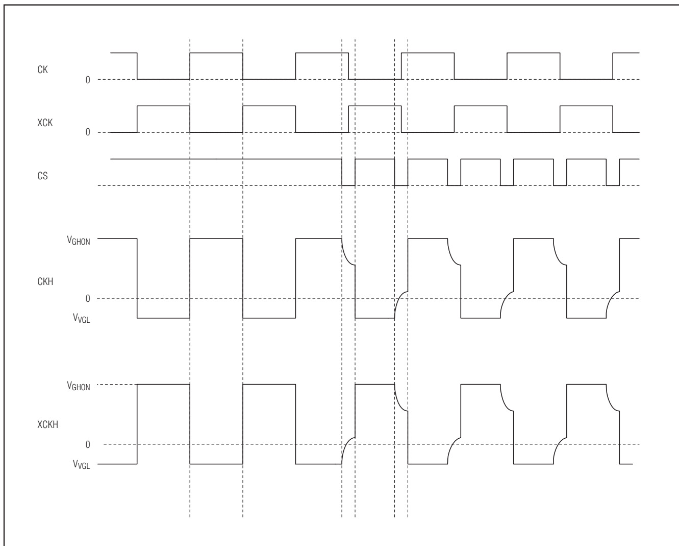
Figure 5. Scan Driver System Timing Utilizing Charge Sharing Between the CKH and XCKH Outputs
