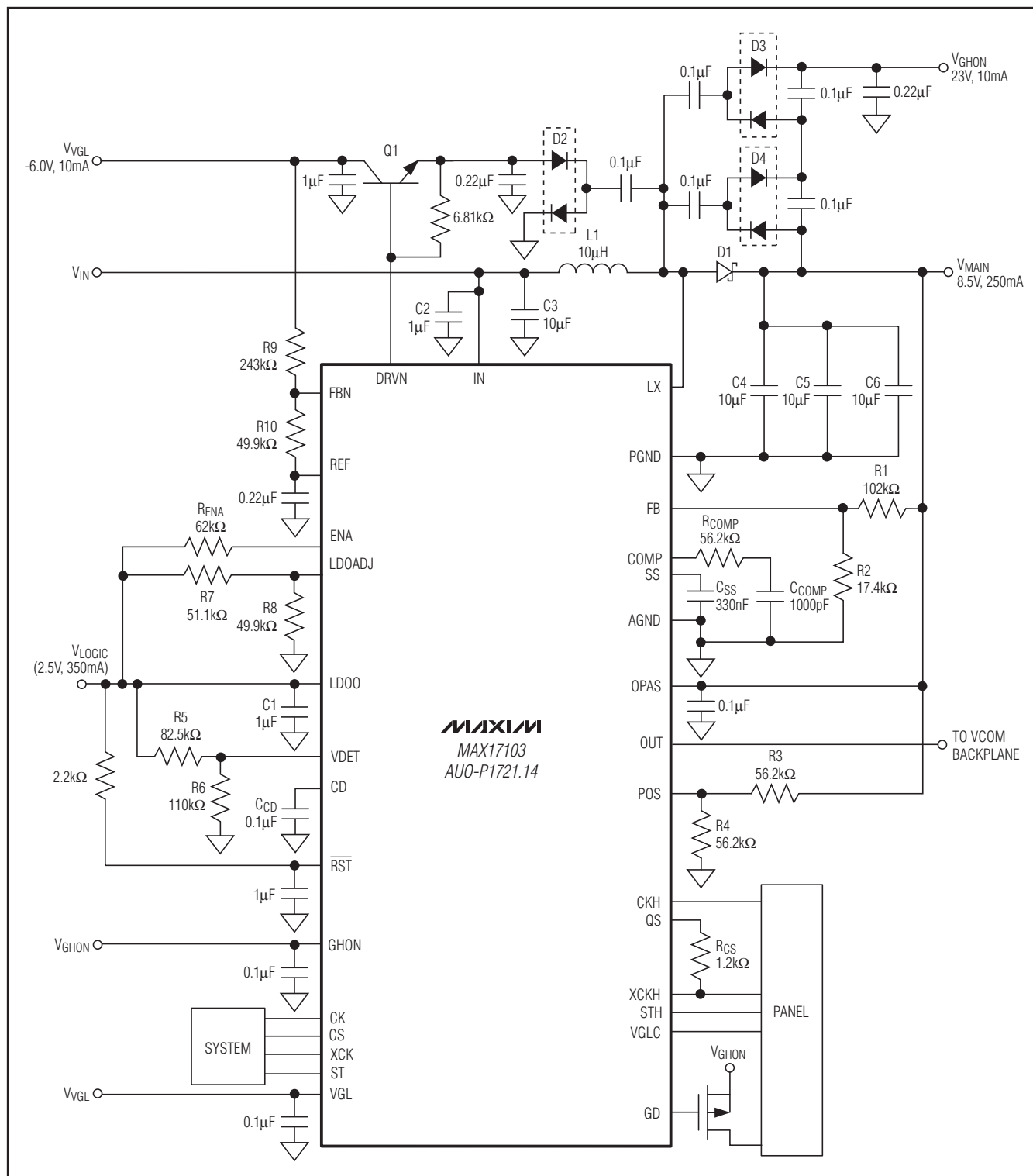
Figure 1. MAX17103 Typical Operating Circuit
