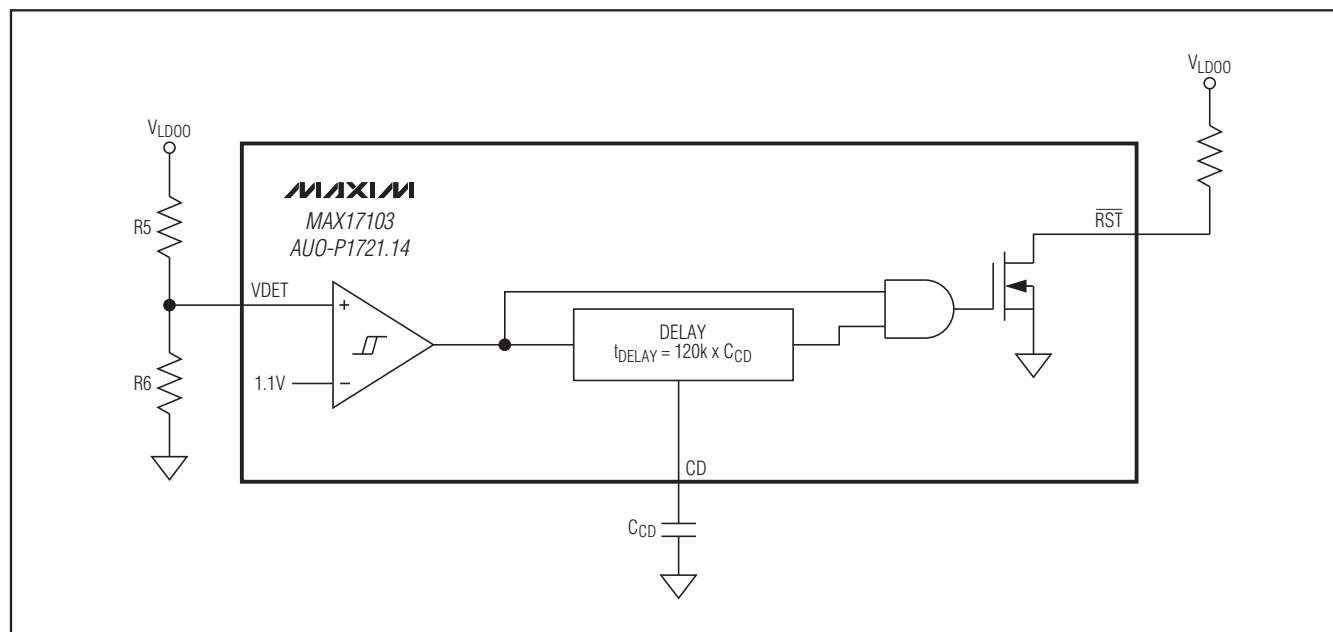
Figure 6. Typical Voltage-Detector Configuration
