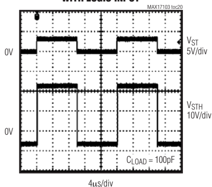
STH OUTPUT WAVEFORM WITH LOGIC INPUT
