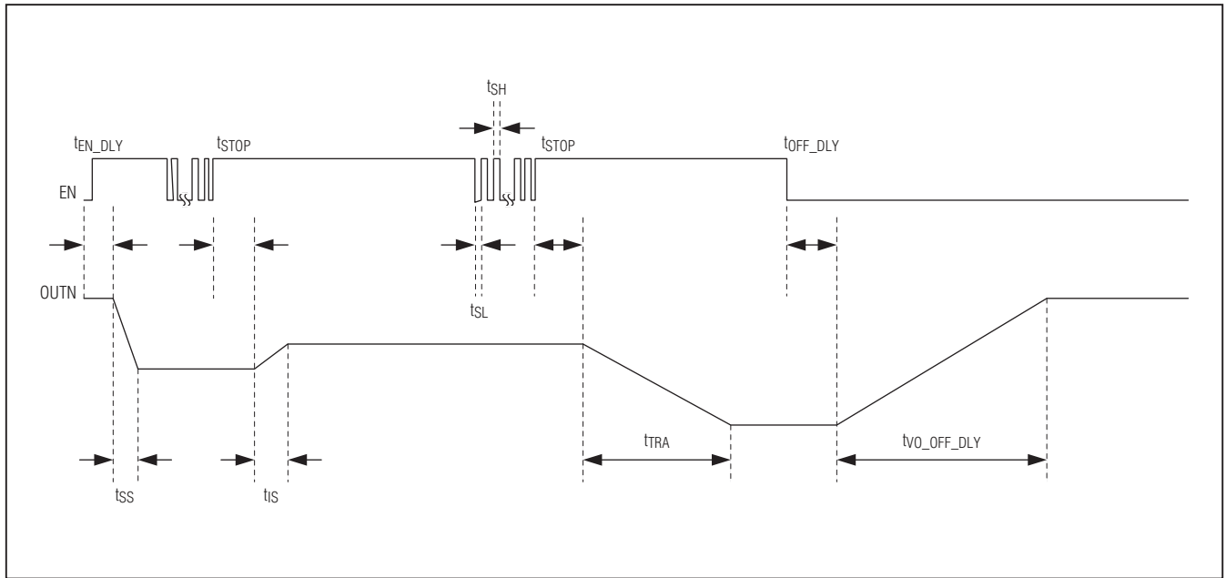
Figure 1. EN Serial Interface Timing Diagram
