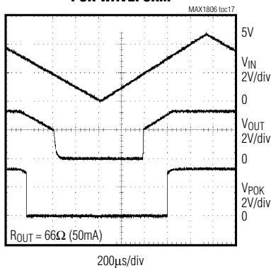
POK WAVEFORM
