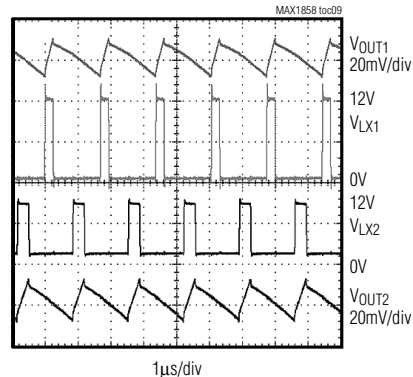
OUT-OF-PHASE WAVEFORM
