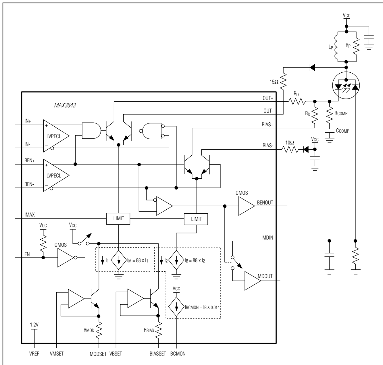
Figure 1. Functional Diagram
