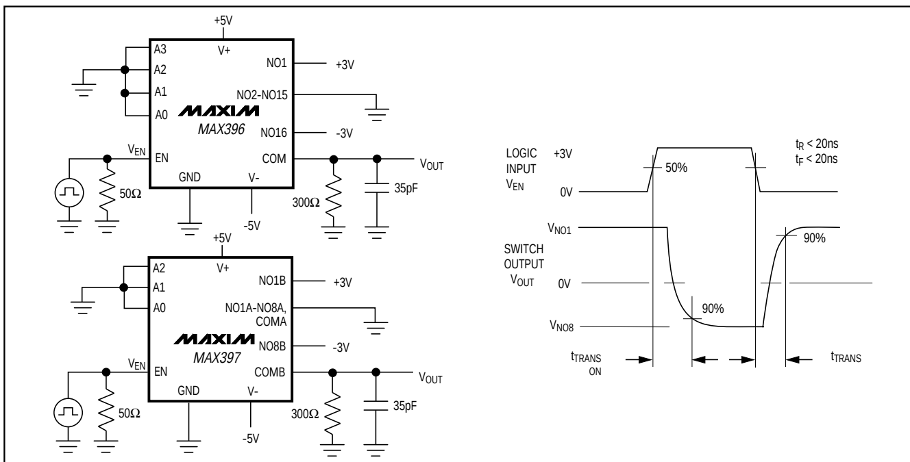
Figure 2. Transition Time
