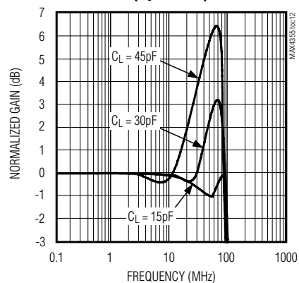
MEDIUM-SIGNAL FREQUENCY RESPONSE ( A_V = +2V/V )
