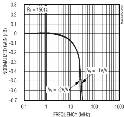
LARGE-SIGNAL GAIN FLATNESS
