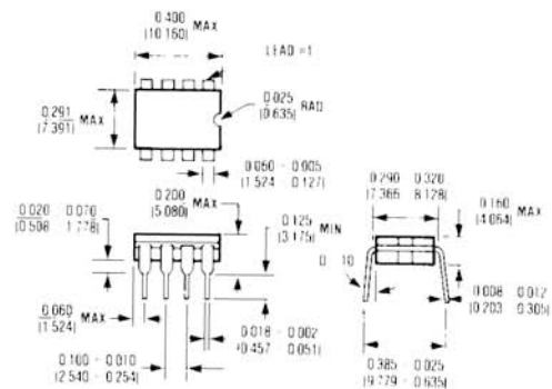
8 Lead Cerdip
