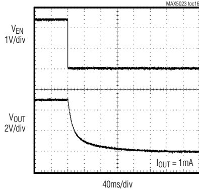
SHUTDOWN RESPONSE
