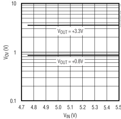
OVERVOLTAGE THRESHOLD (PGOOD) vs. INPUT VOLTAGE
