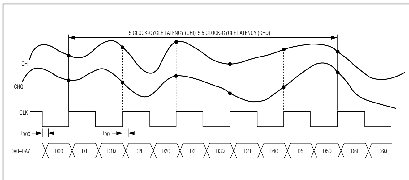
Figure 3. ADC System Timing Diagram
