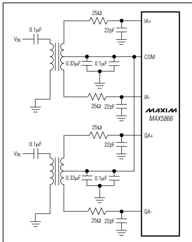
Figure 7. Balun-Transformer-Coupled Single-Ended-to-Differential Input Drive for ADCs
