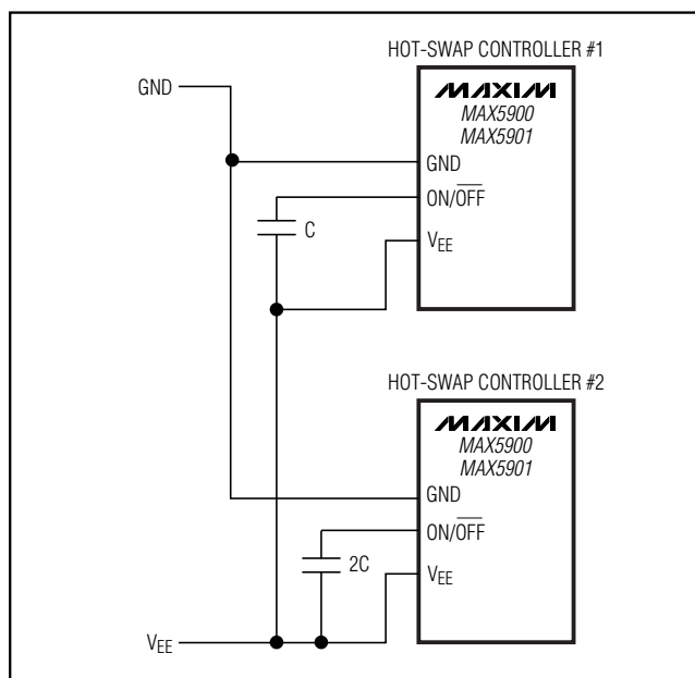
Figure 3. Power-Supply Sequencing
