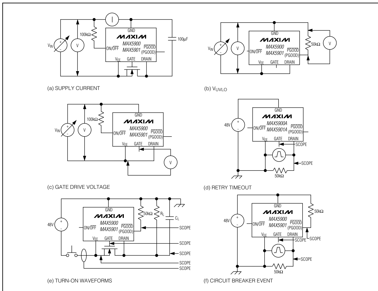
Figure 6. Test Circuits
