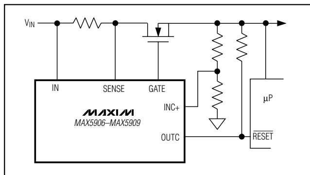
Figure 12. Power-On Reset
