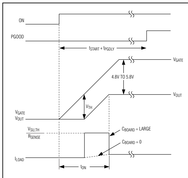
Figure 2. Startup Waveforms
