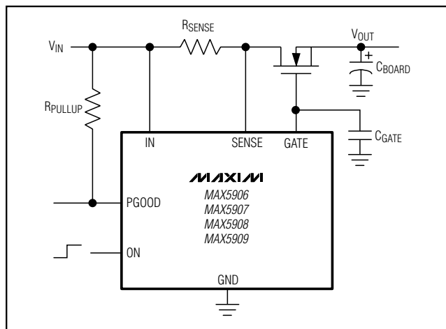
Figure 10. Operating with an External Gate Capacitor
