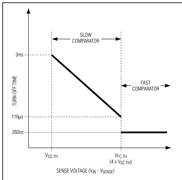
Figure 9. VariableSpeed/BiLevel Response
