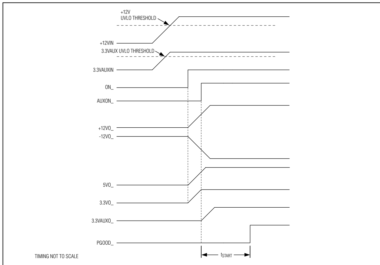
Figure 1. Startup Waveforms
