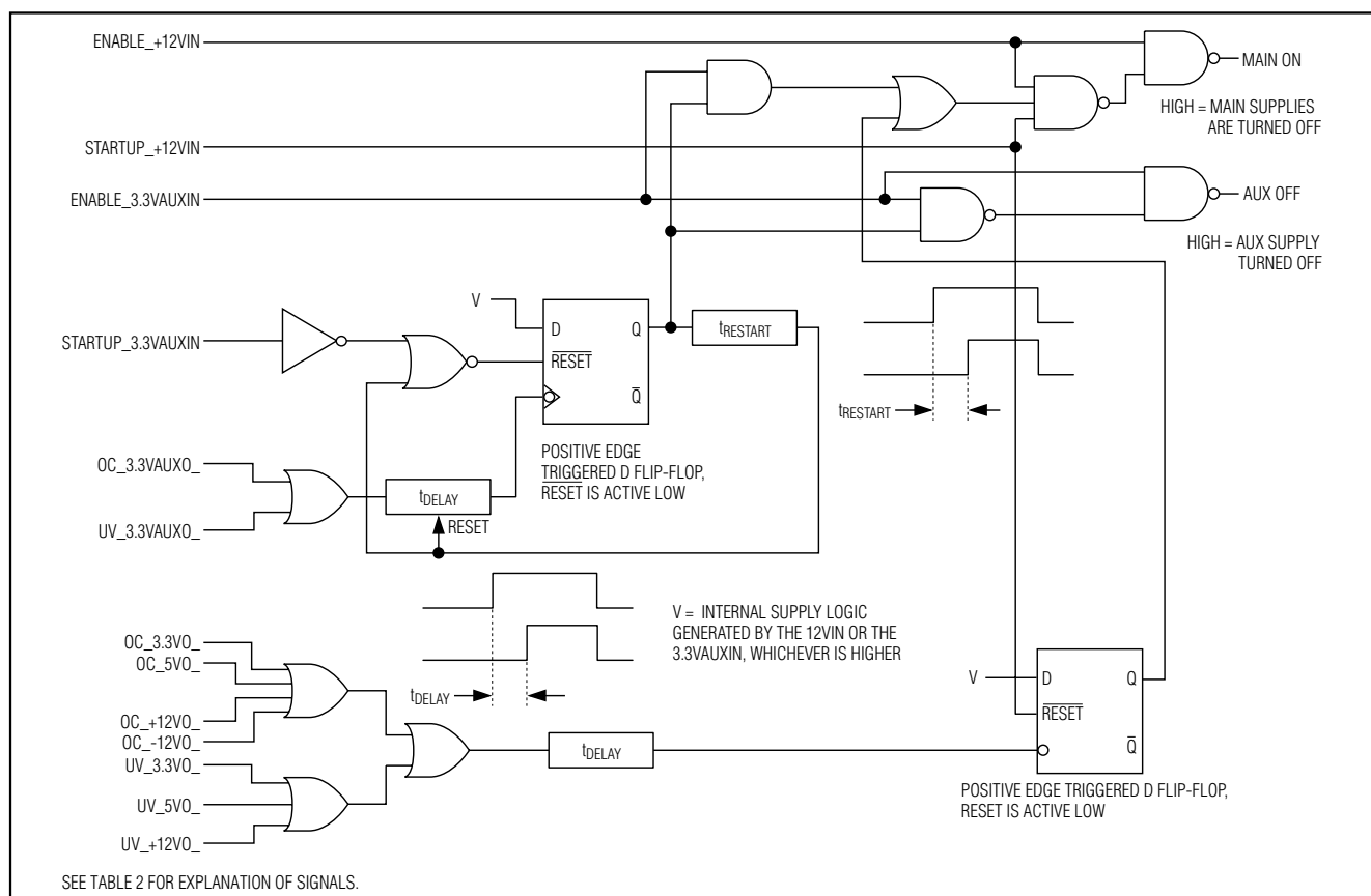
Figure 3. Main and Auxiliary Supply Shutdown Control Logic for MAX5915
