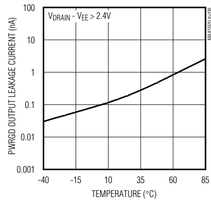
PWRGD OUTPUT LEAKAGE CURRENT vs. TEMPERATURE (MAX5920B)
