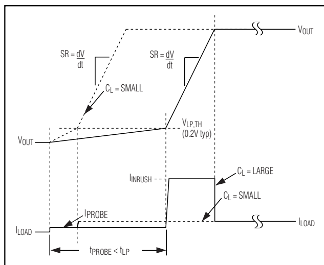
Figure 5. Startup Waveform
