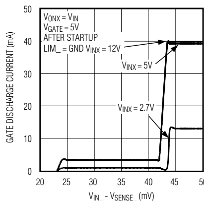
STRONG GATE DISCHARGE CURRENT vs. OVERDRIVE
