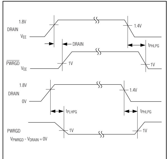
Figure 6. DRAIN to \overline{\text{PWRGD}} /PWRGD Timing
