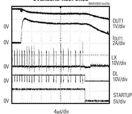
OVERLOAD RESPONSE
