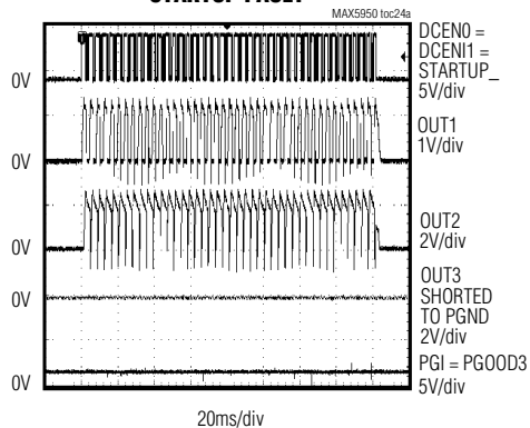
STARTUP FAULT
