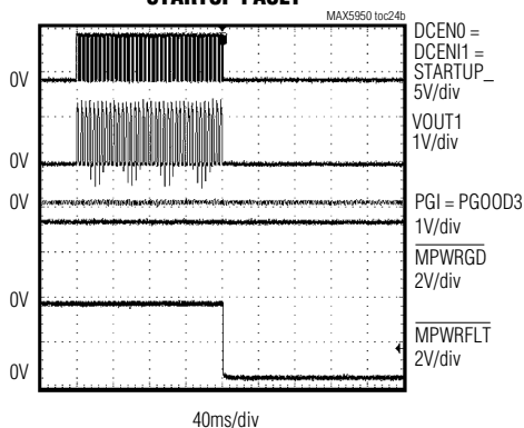
STARTUP FAULT
