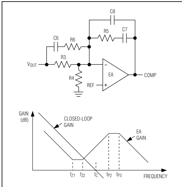
Figure 5. Error-Amplifier Compensation Circuit (Closed-Loop and Error-Amplifier Gain Plot) for Ceramic Capacitors
