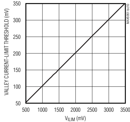
VALLEY CURRENT-LIMIT THRESHOLD vs. V_{ILIM}
