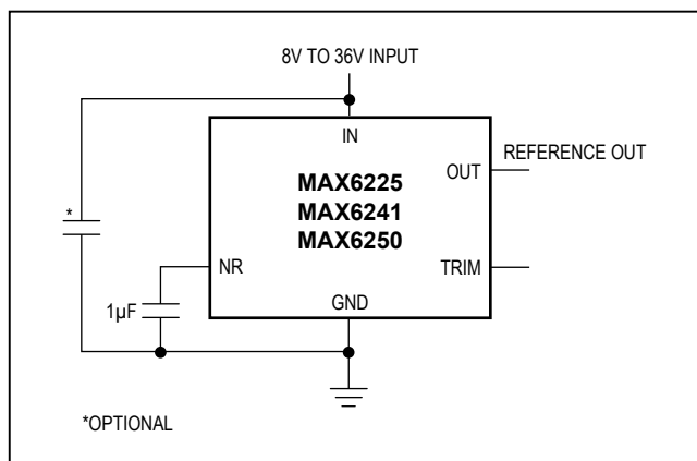
Figure 2. Noise-Reduction Capacitor
