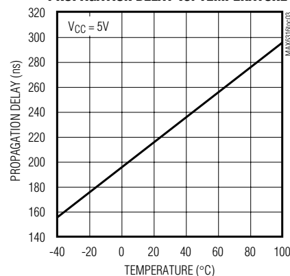
MAX6316/MAX6317/MAX6319/MAX6320/MAX6322 MANUAL RESET TO RESET PROPAGATION DELAY vs. TEMPERATURE
