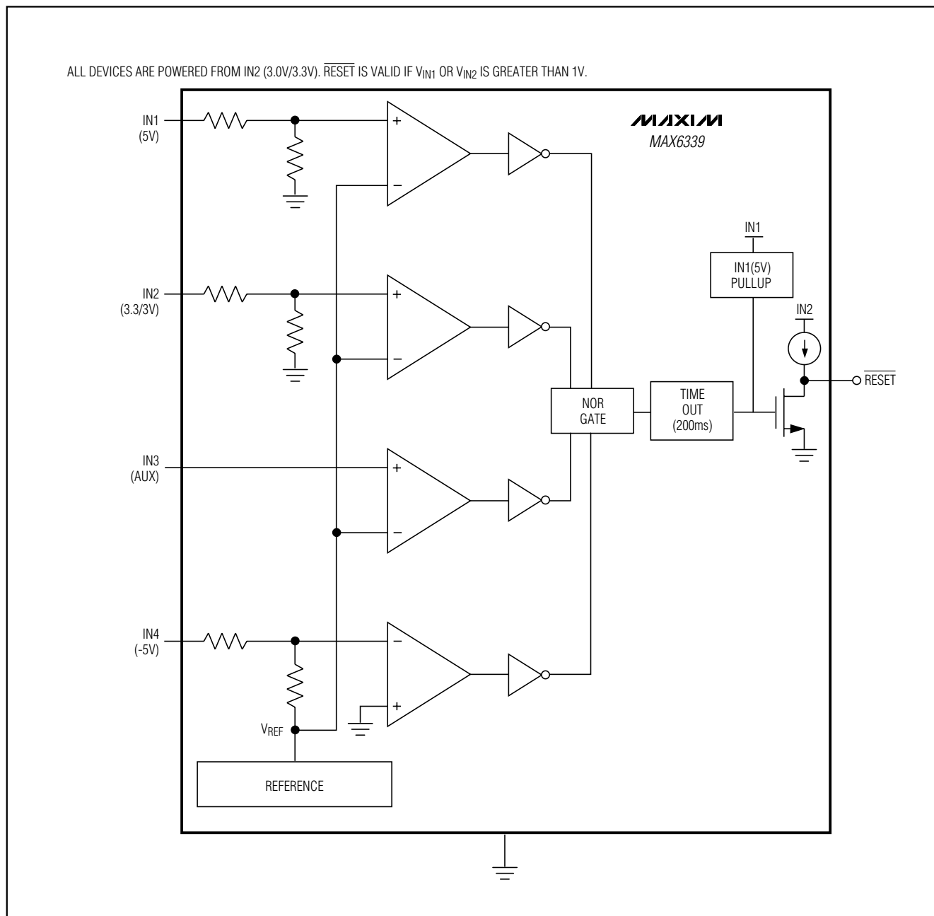
Figure 1. MAX6339 Functional Diagram
