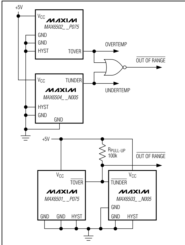
Figure 4. Temperature-Window Alarms
