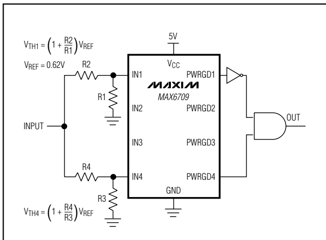
Figure 5. Window Detection
