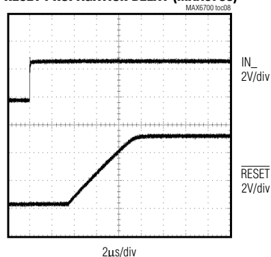
RESET PROPAGATION DELAY (MAX6700)
