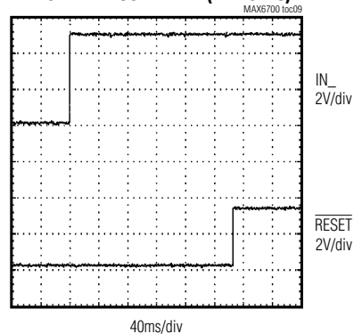
RESET TIMEOUT DELAY (MAX6710)
