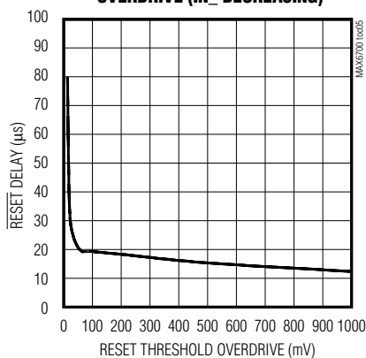
RESET DELAY vs. RESET THRESHOLD OVERDRIVE (IN 1 DECREASING)
