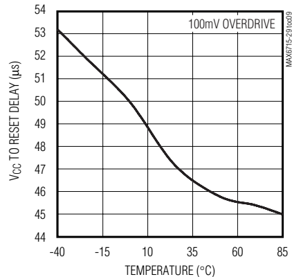
V_{CC} TO RESET DELAY vs. TEMPERATURE
