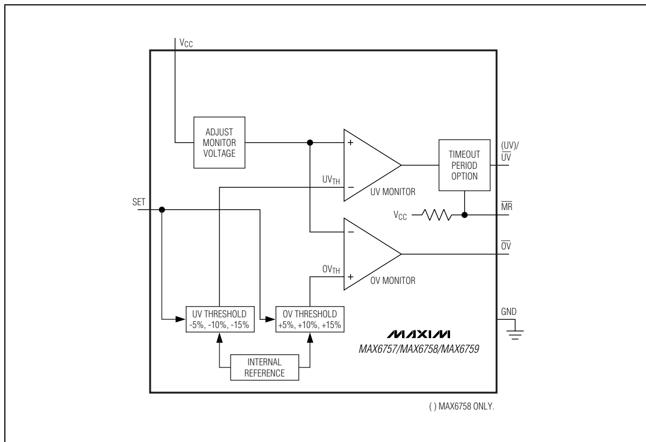
Figure 2. MAX6757/MAX6758/MAX6759 Functional Diagram
