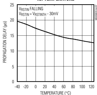
V RSTIN TO RESET OUTPUT DELAY vs. TEMPERATURE
