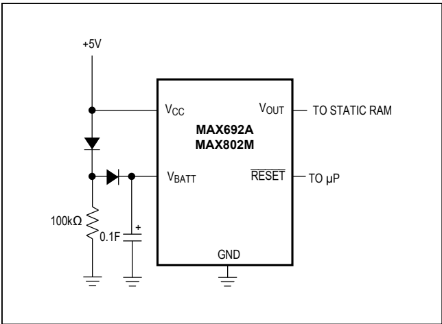
Figure 5. Using a SuperCap as a Backup Power Source with the MAX692A/MAX802M and a +5V ±10% Supply When V BATT connects to V OUT , backup mode is activated and the internal circuitry is powered from the battery (Table 1). When V CC is just below V BATT , the current drawn from V BATT is typically 30μA. When V CC drops to more than 1V below V BATT , the internal switchover comparator shuts off and the supply current falls to less than 1μA.
