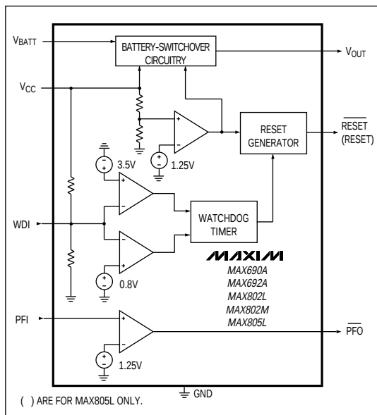
Figure 1. Block Diagram
