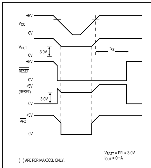
Figure 2. Timing Diagram
