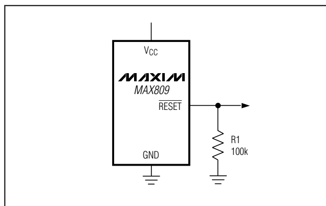
Figure 2. \overline{\text{RESET}} Valid to V_{CC} = \text{Ground} Circuit
