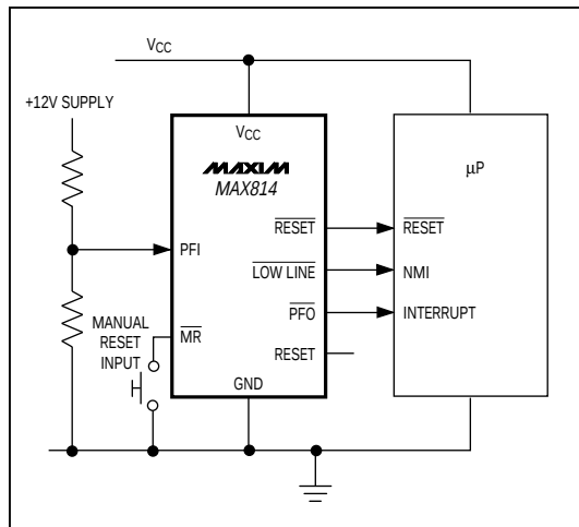
Figure 1b. MAX814 Typical Application
