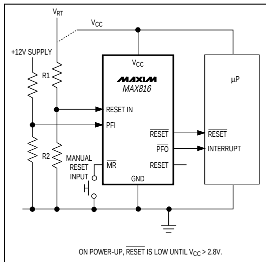
Figure 3. MAX816 Typical Application
