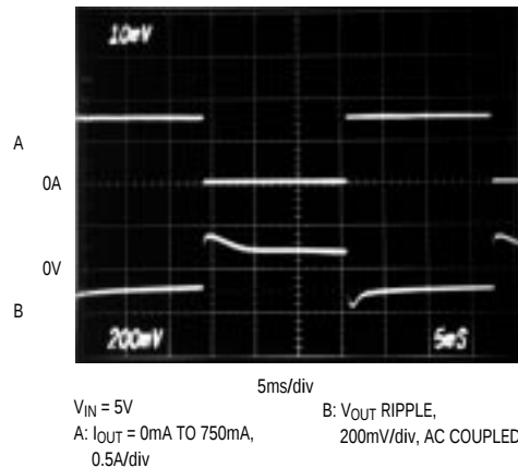
LOAD-TRANSIENT RESPONSE
